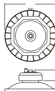
George 24000lm & 30000lm Dimensions (mm)
