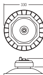
George 12000lm & 18000lm Dimensions (mm)
